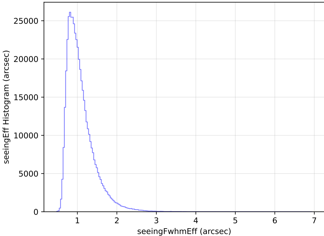
scp_reweight_v3.3_10yrs WFD i band: seeingEff Histogram
