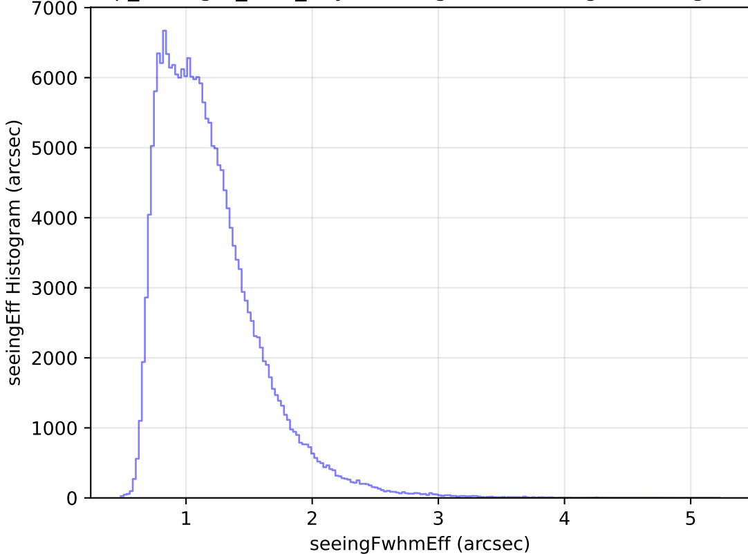
scp_reweight_v3.3_10yrs WFD g band: seeingEff Histogram
