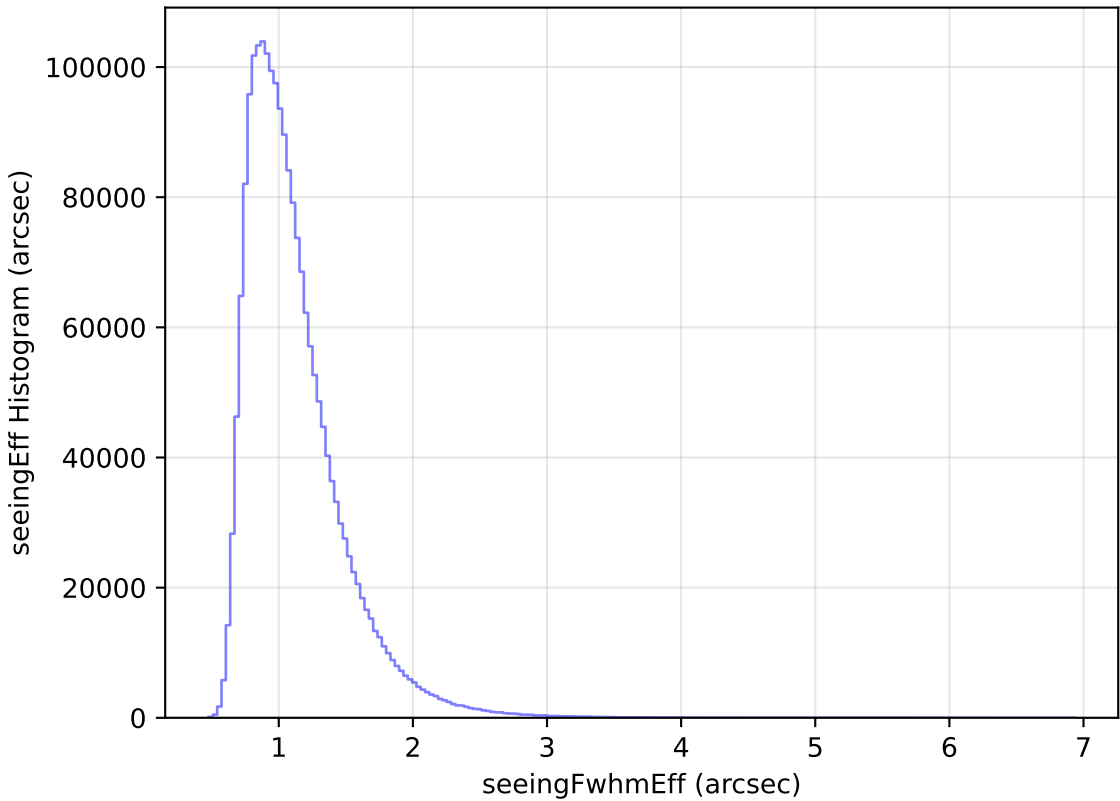
scp_reweight_v3.3_10yrs WFD all bands: seeingEff Histogram
