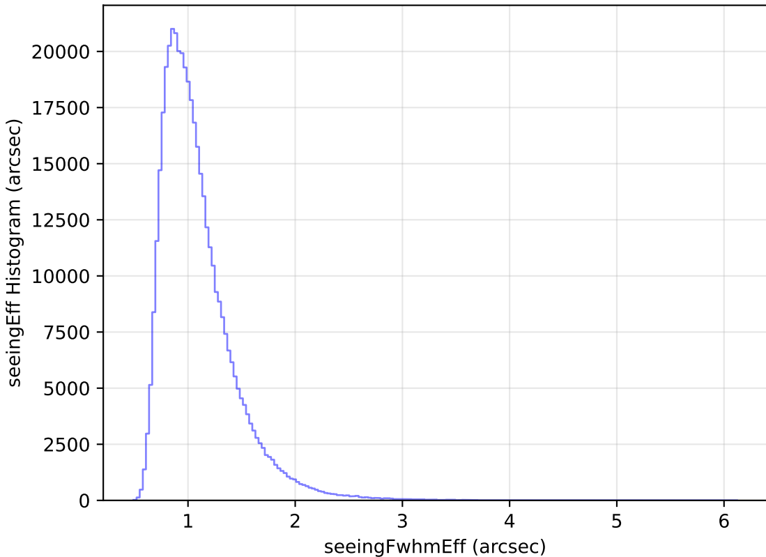
scp_reweight_v3.3_10yrs All sky z band: seeingEff Histogram
