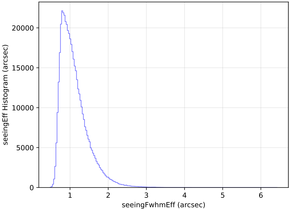
scp_reweight_v3.3_10yrs All sky r band: seeingEff Histogram
