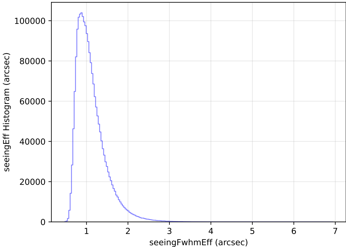
scp_reweight_v3.3_10yrs All sky all bands: seeingEff Histogram
