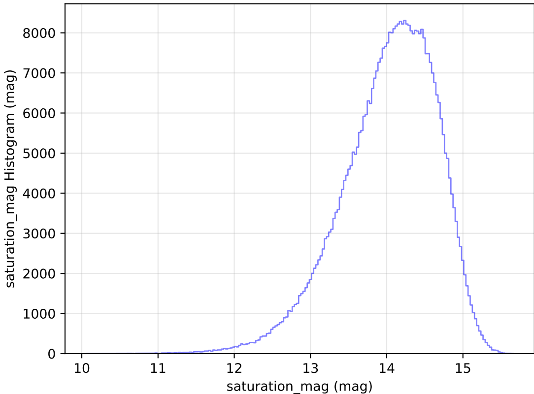
scp_reweight_v3.3_10yrs WFD z band: saturation_mag Histogram
