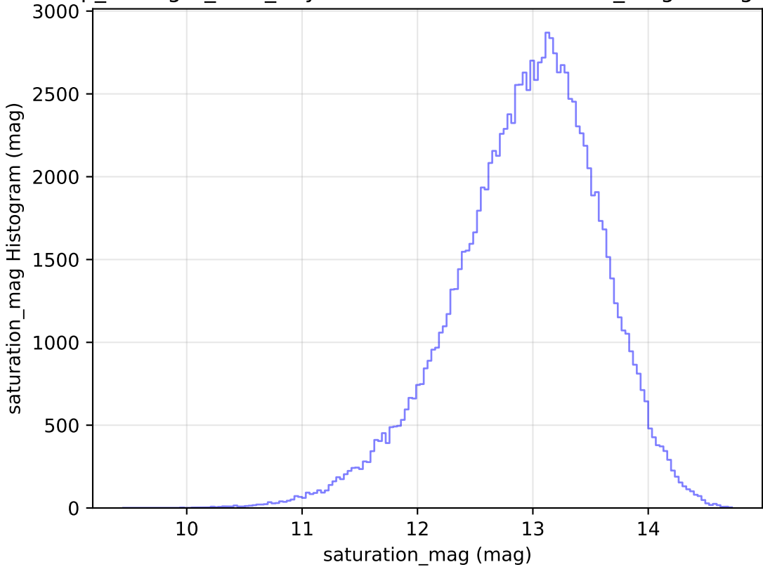
scp_reweight_v3.3_10yrs WFD u band: saturation_mag Histogram
