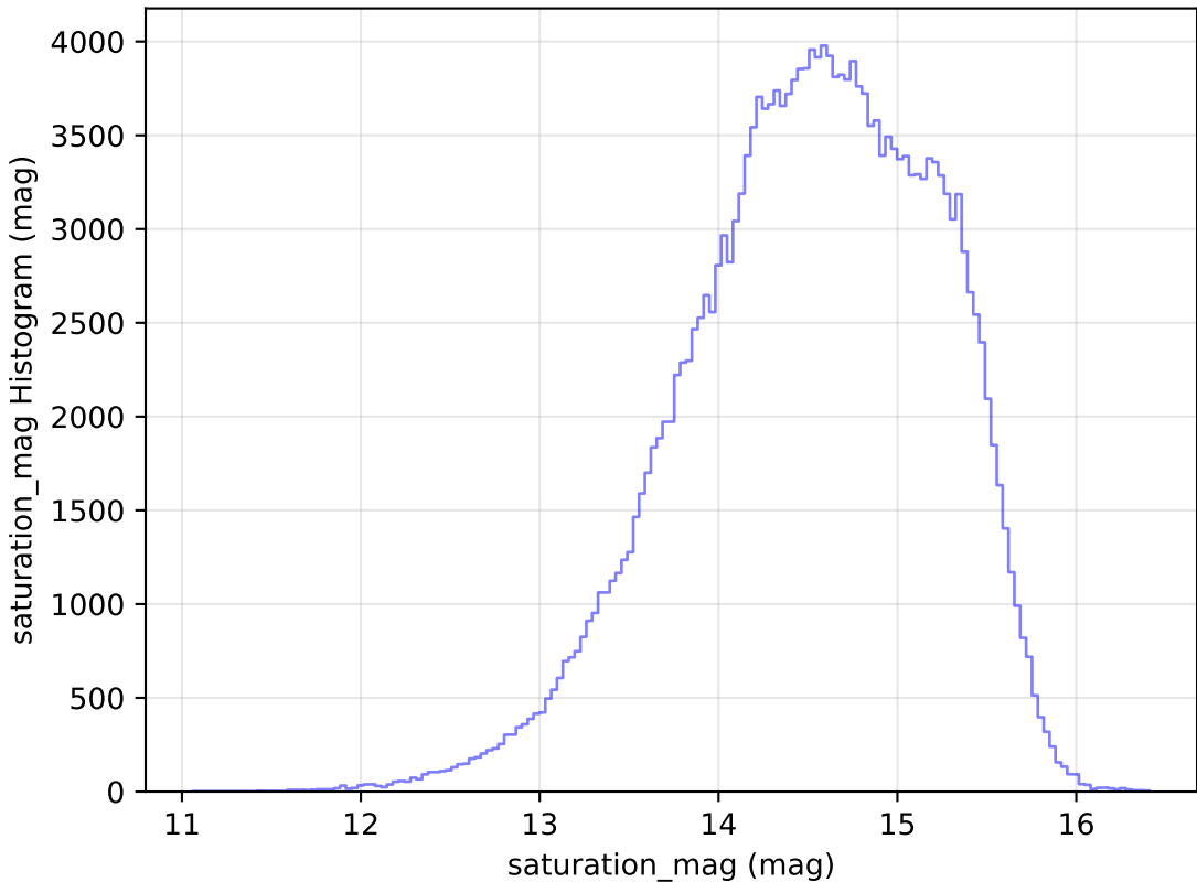
scp_reweight_v3.3_10yrs WFD g band: saturation_mag Histogram
