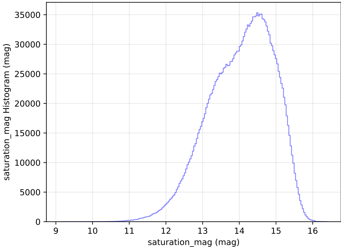
scp_reweight_v3.3_10yrs WFD all bands: saturation_mag Histogram
