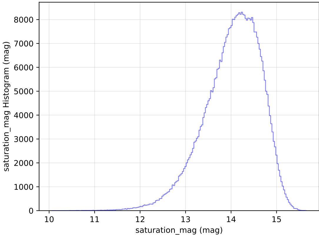
scp_reweight_v3.3_10yrs All sky z band: saturation_mag Histogram
