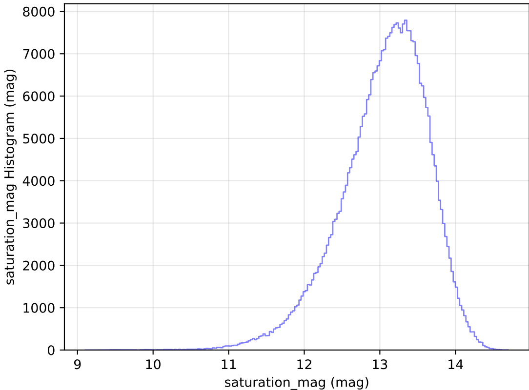
scp_reweight_v3.3_10yrs All sky y band: saturation_mag Histogram
