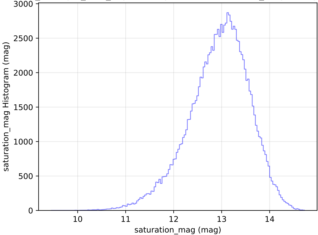
scp_reweight_v3.3_10yrs All sky u band: saturation_mag Histogram
