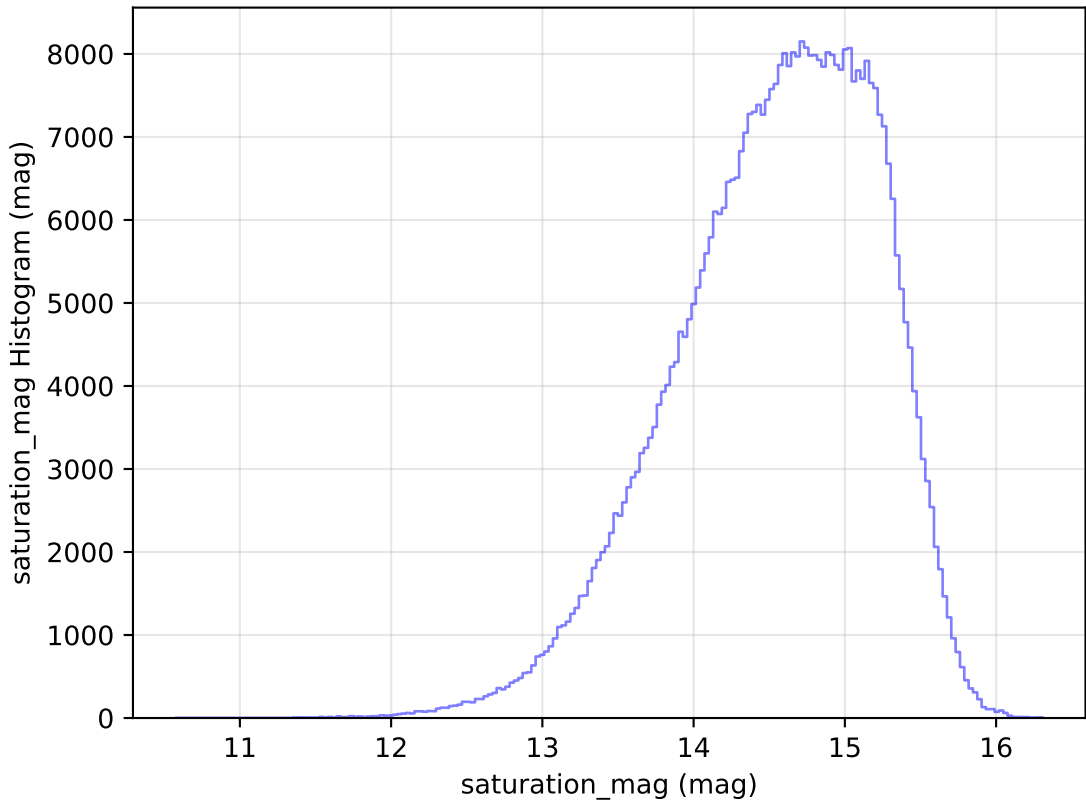
scp_reweight_v3.3_10yrs All sky r band: saturation_mag Histogram
