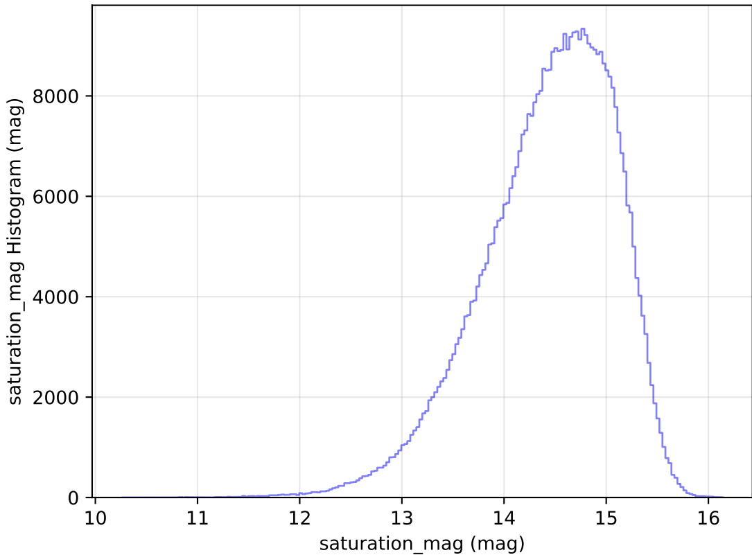
scp_reweight_v3.3_10yrs All sky i band: saturation_mag Histogram
