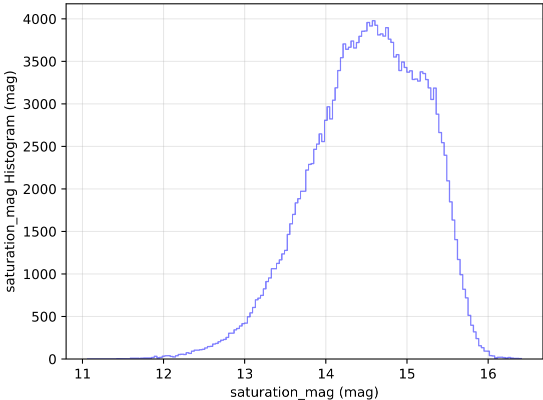
scp_reweight_v3.3_10yrs All sky g band: saturation_mag Histogram
