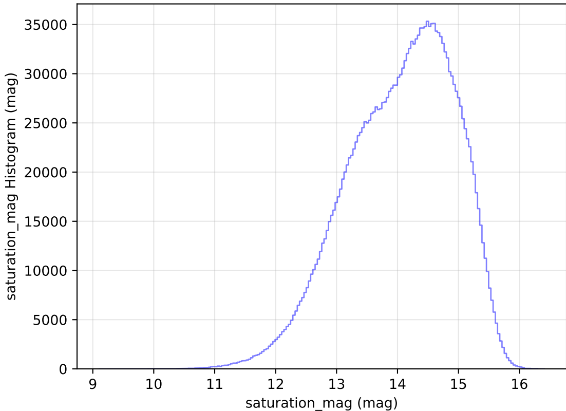
scp_reweight_v3.3_10yrs All sky all bands: saturation_mag Histogram
