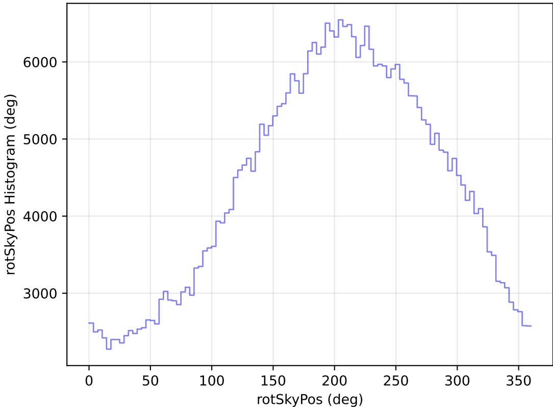
scp_reweight_v3.3_10yrs WFD z band: rotSkyPos Histogram
