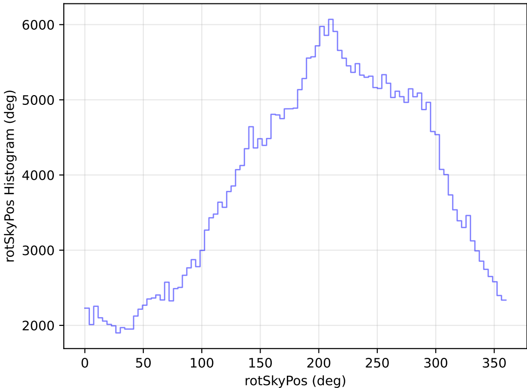
scp_reweight_v3.3_10yrs WFD y band: rotSkyPos Histogram
