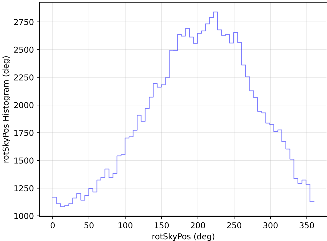
scp_reweight_v3.3_10yrs WFD u band: rotSkyPos Histogram
