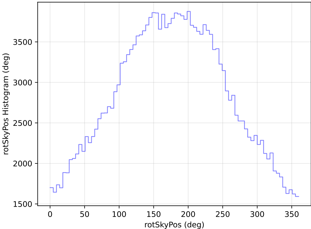
scp_reweight_v3.3_10yrs WFD g band: rotSkyPos Histogram
