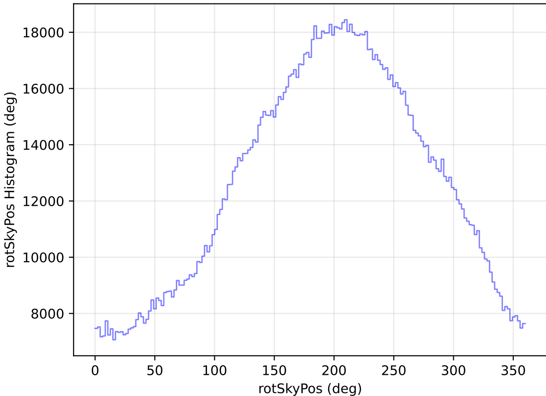
scp_reweight_v3.3_10yrs WFD all bands: rotSkyPos Histogram
