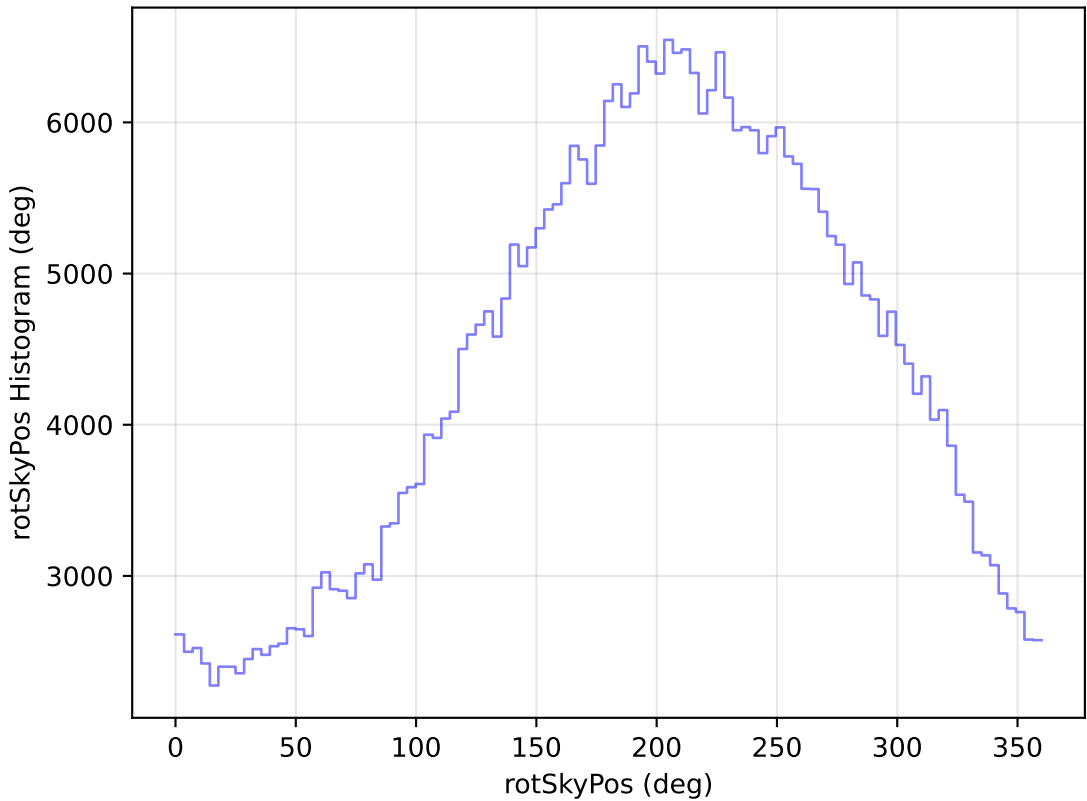
scp_reweight_v3.3_10yrs All sky z band: rotSkyPos Histogram
