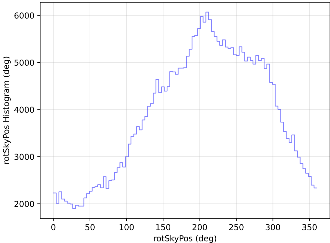
scp_reweight_v3.3_10yrs All sky y band: rotSkyPos Histogram
