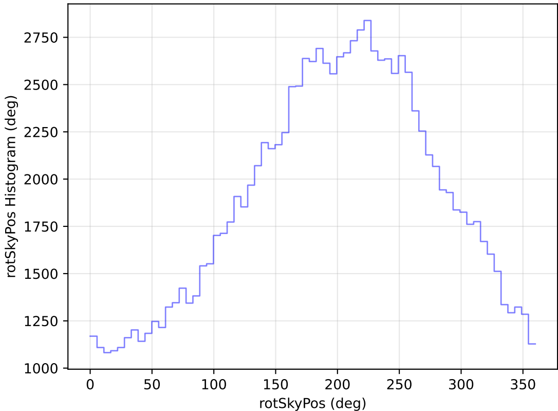
scp_reweight_v3.3_10yrs All sky u band: rotSkyPos Histogram
