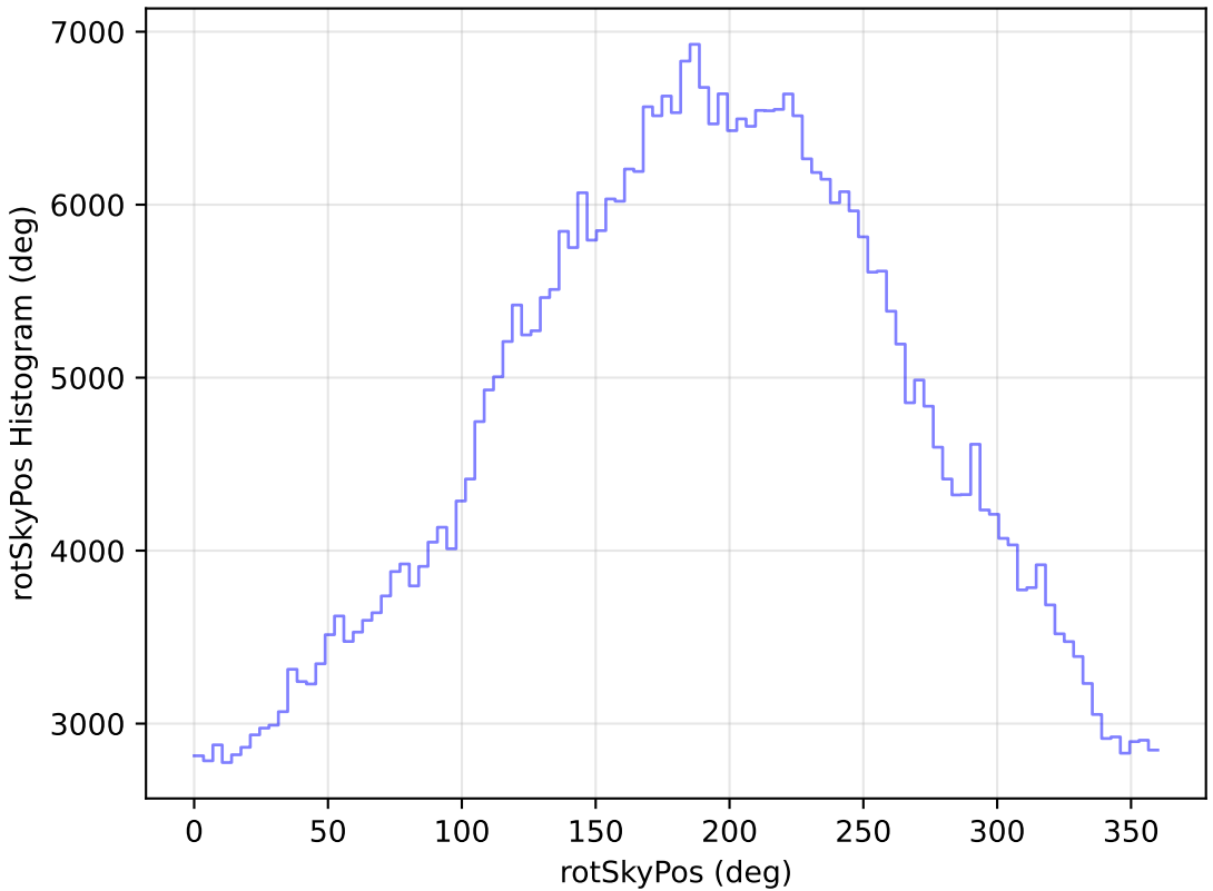
scp_reweight_v3.3_10yrs All sky r band: rotSkyPos Histogram
