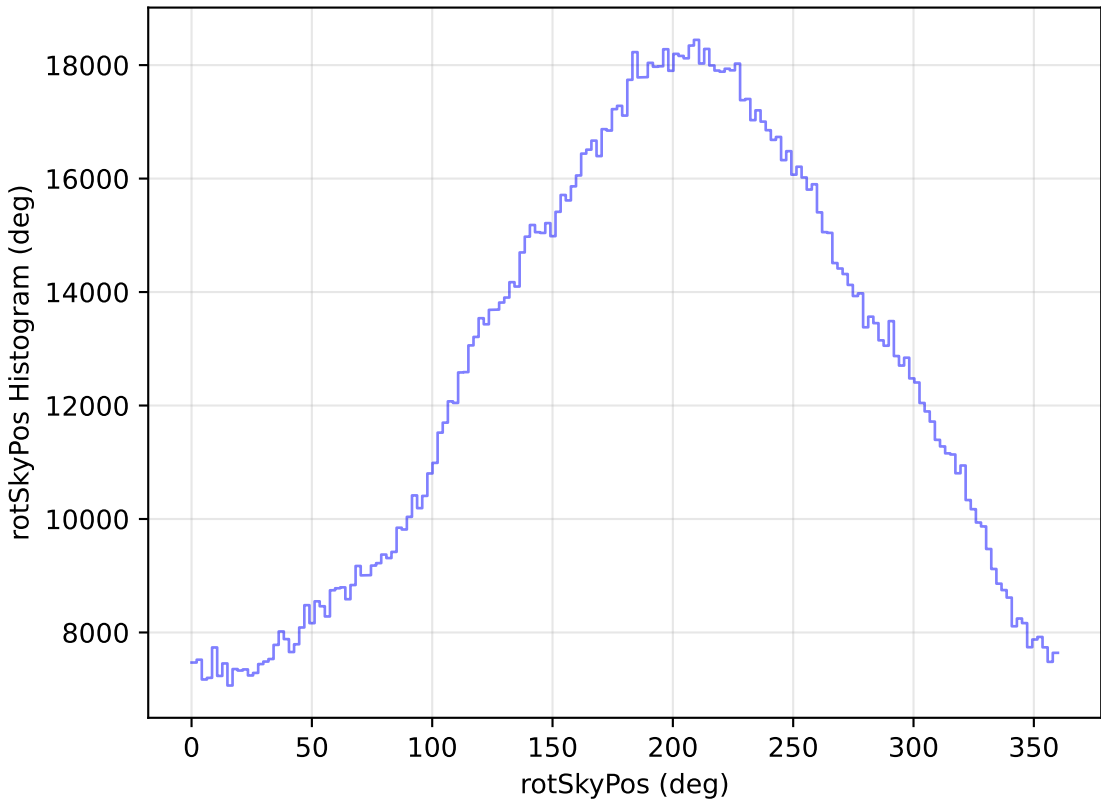
scp_reweight_v3.3_10yrs All sky all bands: rotSkyPos Histogram
