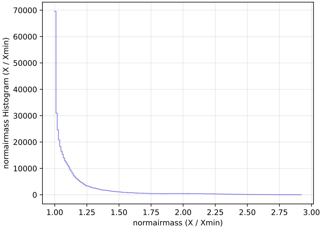
scp_reweight_v3.3_10yrs WFD z band: normairmass Histogram
