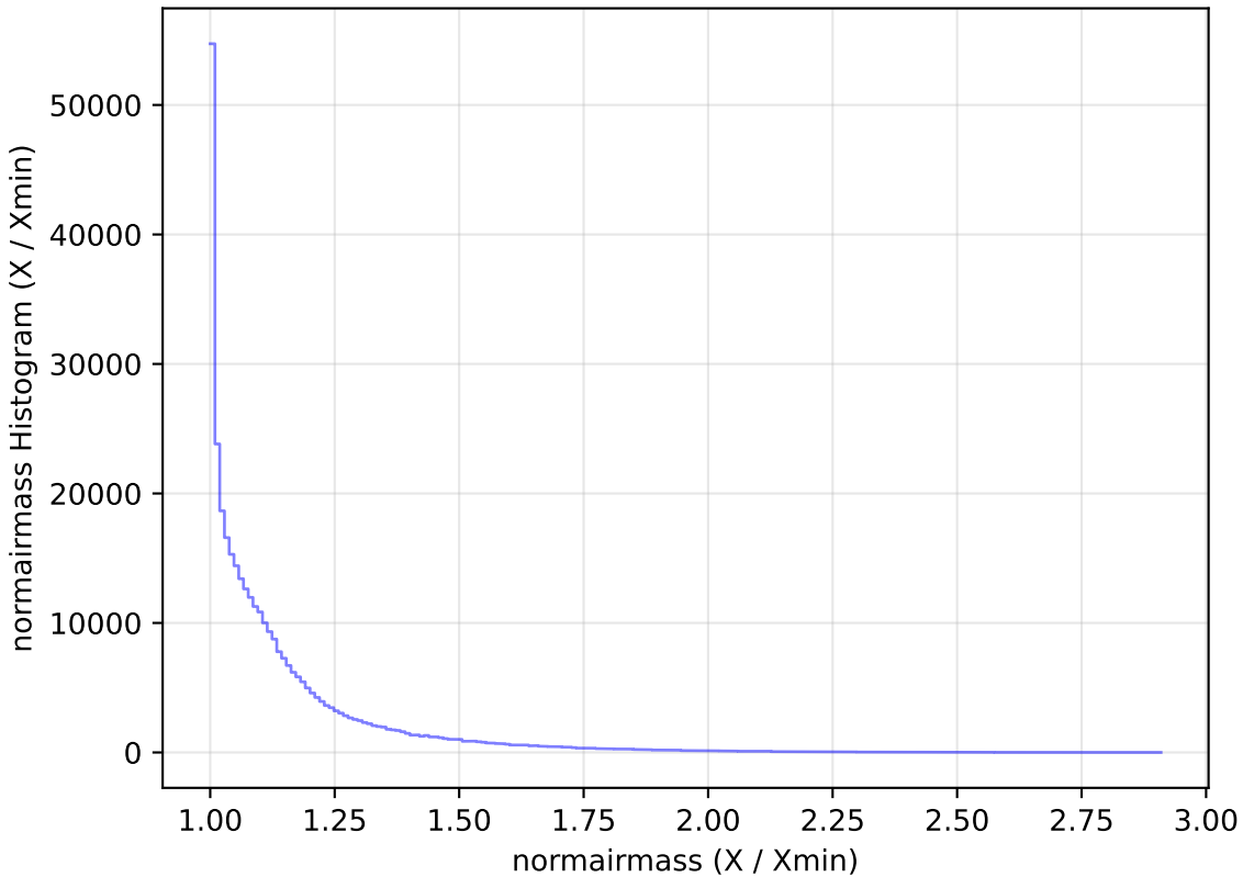
scp_reweight_v3.3_10yrs WFD y band: normairmass Histogram
