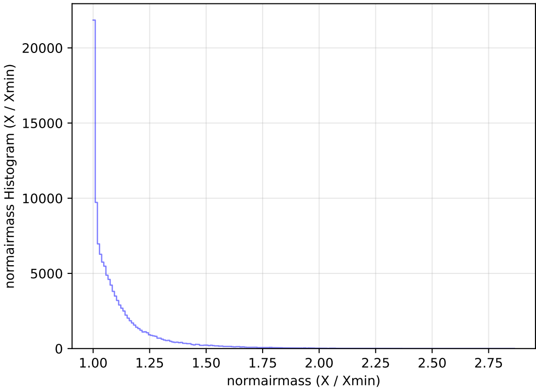
scp_reweight_v3.3_10yrs WFD u band: normairmass Histogram
