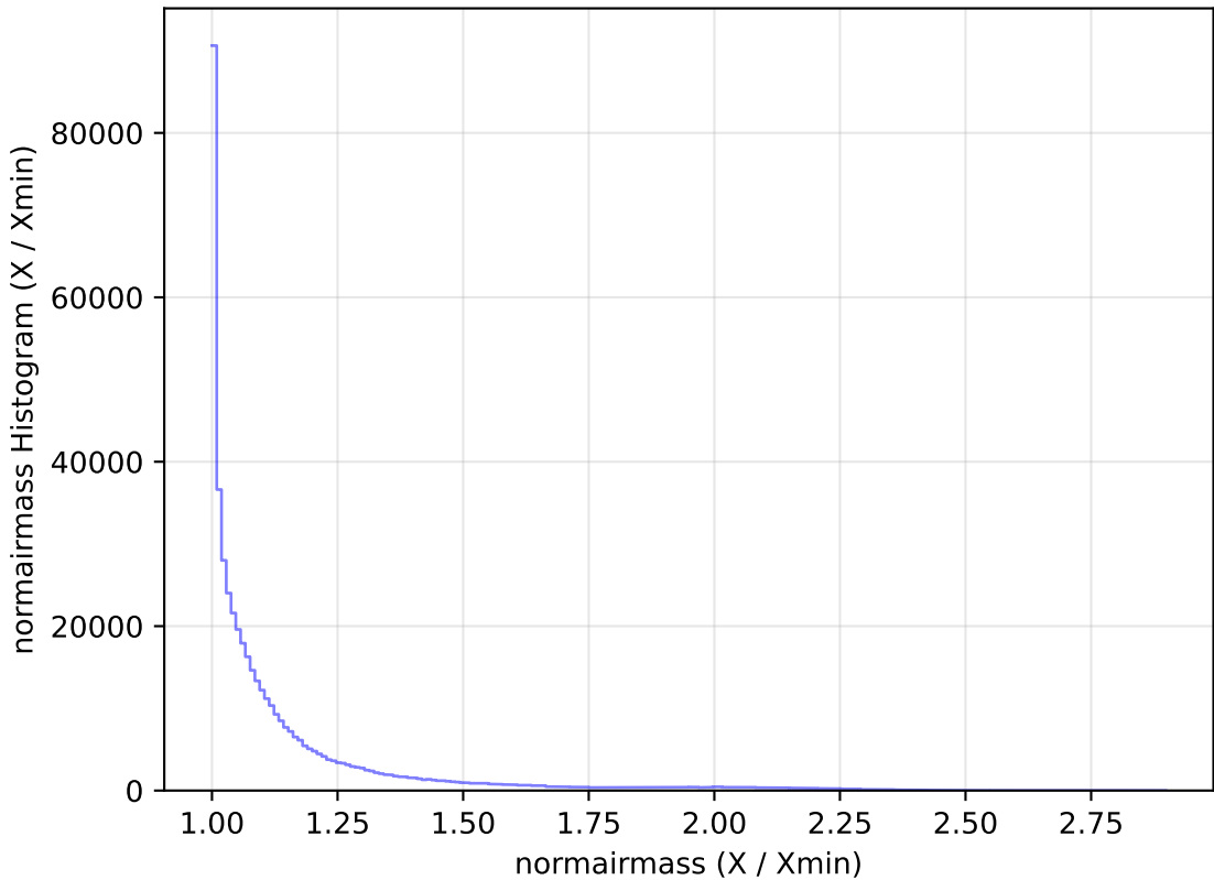
scp_reweight_v3.3_10yrs WFD r band: normairmass Histogram
