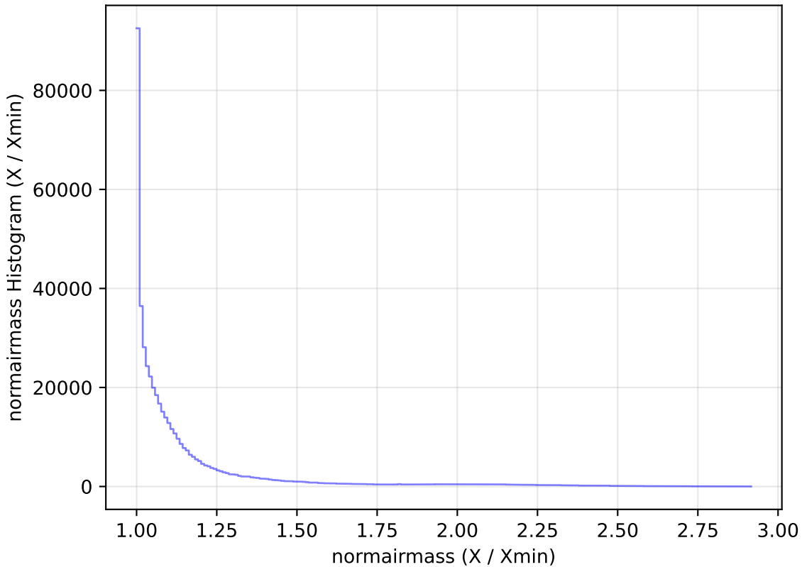
scp_reweight_v3.3_10yrs WFD i band: normairmass Histogram
