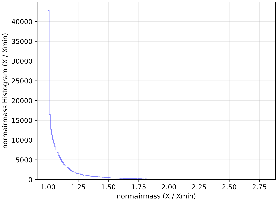
scp_reweight_v3.3_10yrs WFD g band: normairmass Histogram
