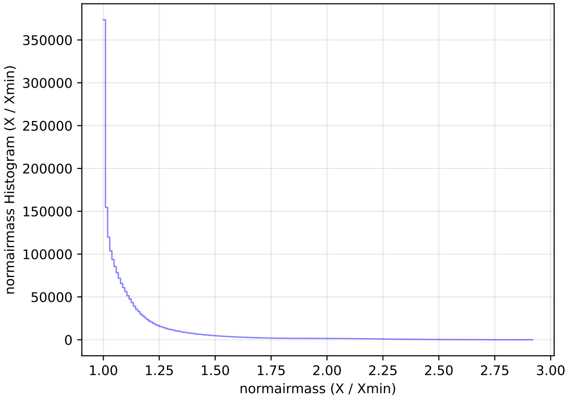
scp_reweight_v3.3_10yrs WFD all bands: normairmass Histogram
