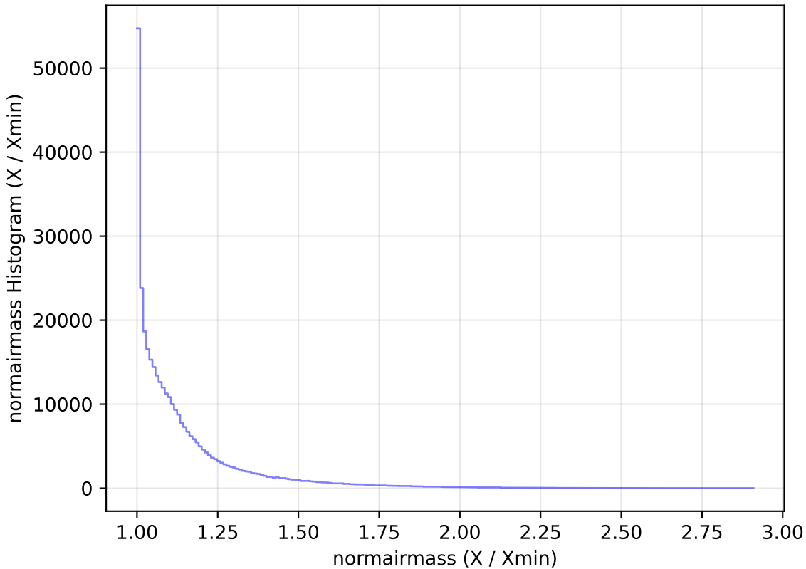
scp_reweight_v3.3_10yrs All sky y band: normairmass Histogram
