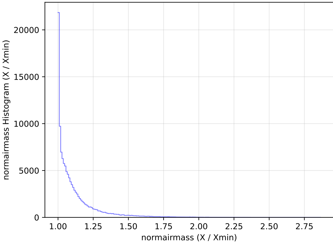
scp_reweight_v3.3_10yrs All sky u band: normairmass Histogram
