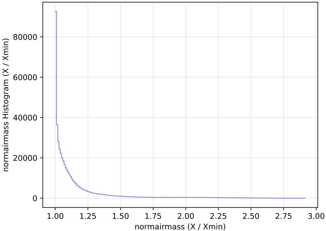
scp_reweight_v3.3_10yrs All sky i band: normairmass Histogram
