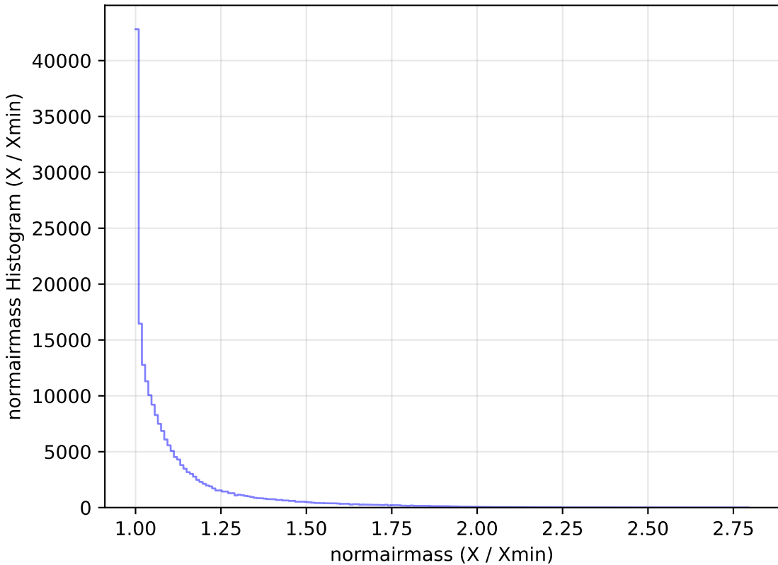
scp_reweight_v3.3_10yrs All sky g band: normairmass Histogram
