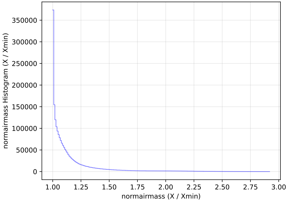
scp_reweight_v3.3_10yrs All sky all bands: normairmass Histogram
