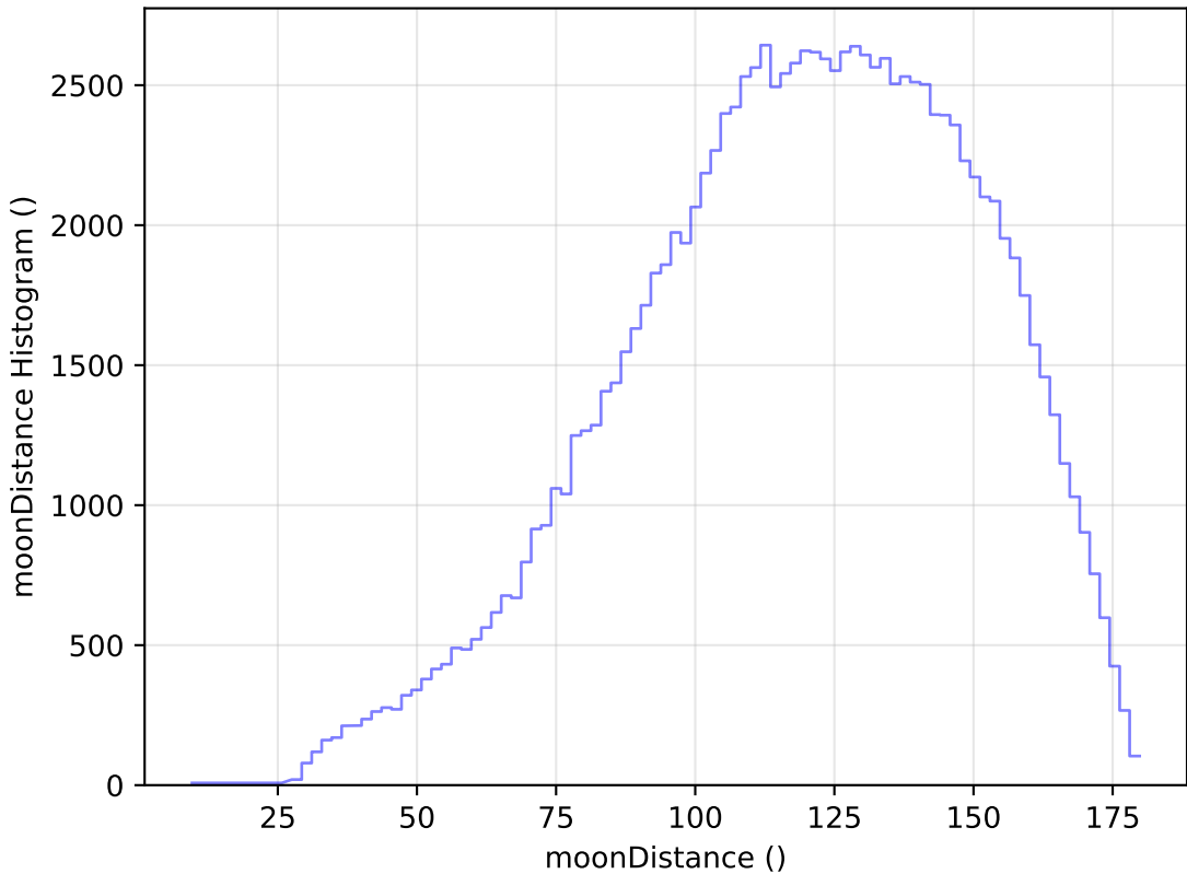
scp_reweight_v3.3_10yrs WFD u band: moonDistance Histogram
