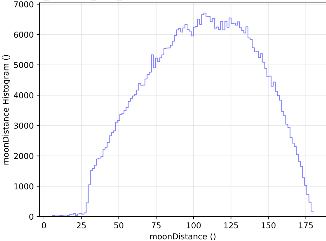
scp_reweight_v3.3_10yrs WFD r band: moonDistance Histogram
