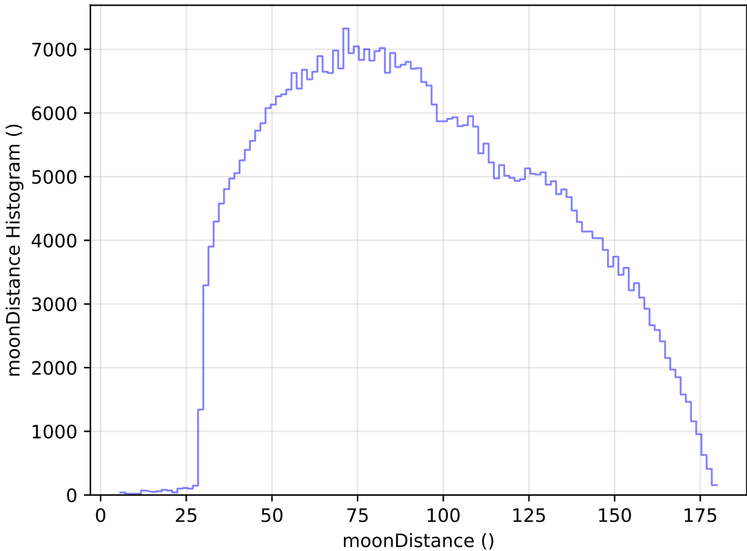
scp_reweight_v3.3_10yrs WFD i band: moonDistance Histogram
