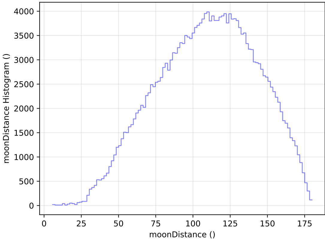
scp_reweight_v3.3_10yrs WFD g band: moonDistance Histogram
