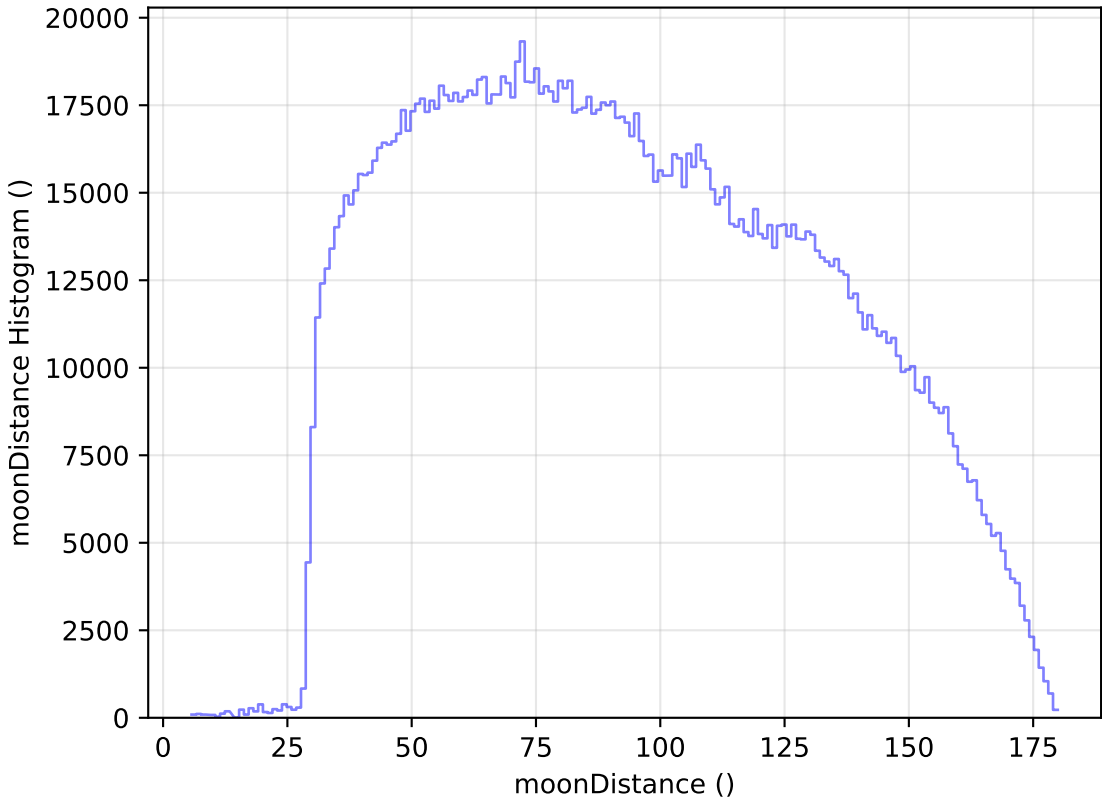
scp_reweight_v3.3_10yrs WFD all bands: moonDistance Histogram
