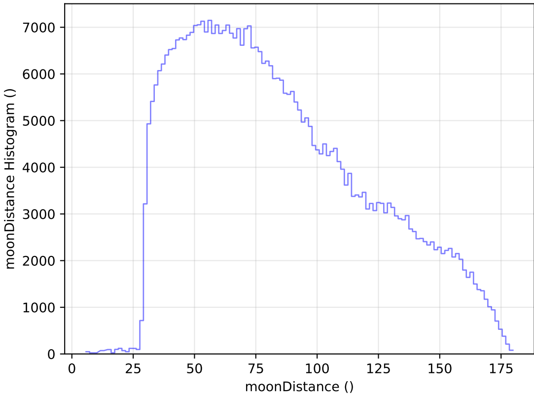
scp_reweight_v3.3_10yrs All sky z band: moonDistance Histogram
