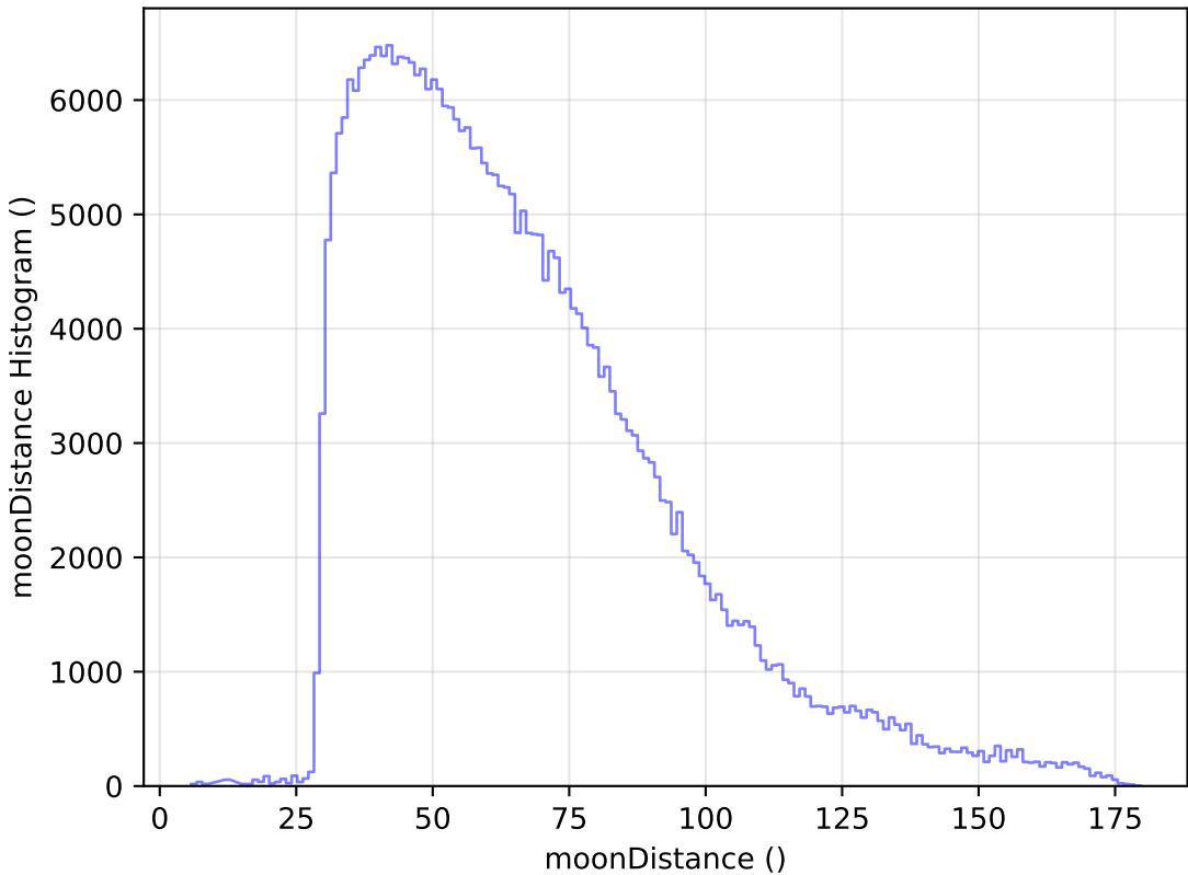
scp_reweight_v3.3_10yrs All sky y band: moonDistance Histogram
