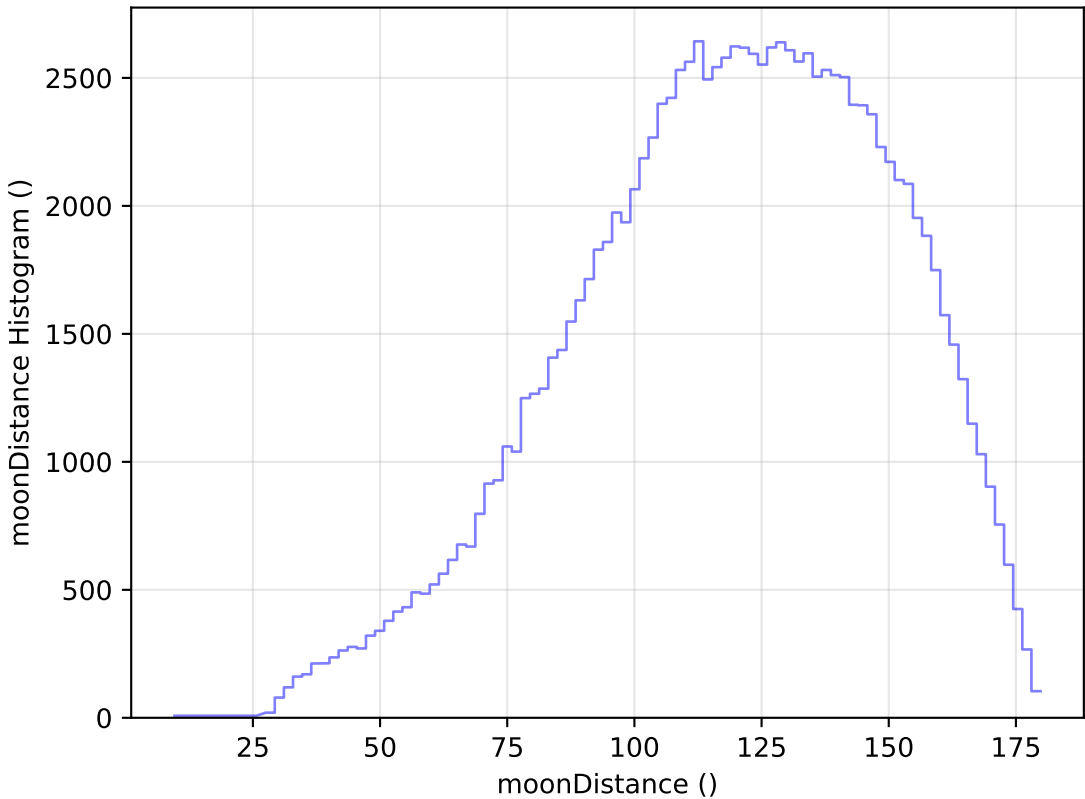
scp_reweight_v3.3_10yrs All sky u band: moonDistance Histogram
