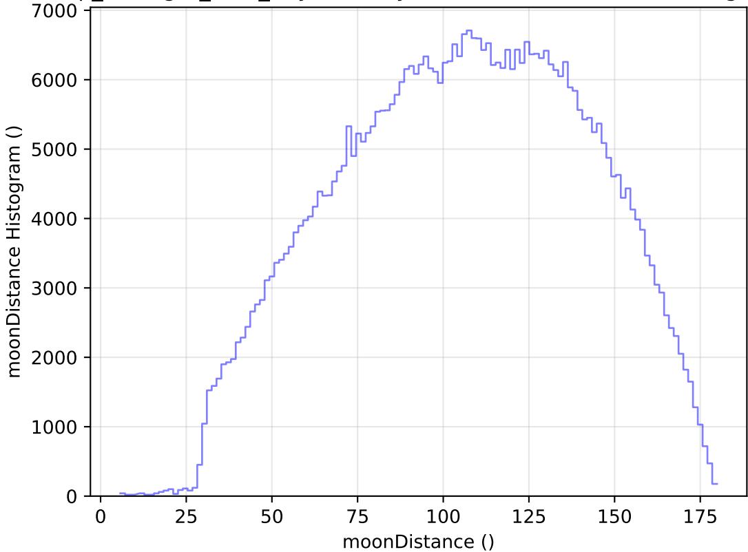
scp_reweight_v3.3_10yrs All sky r band: moonDistance Histogram
