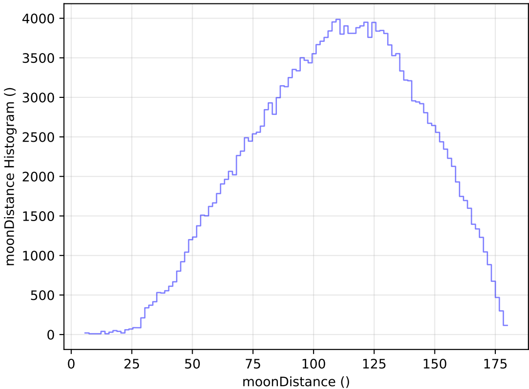
scp_reweight_v3.3_10yrs All sky g band: moonDistance Histogram
