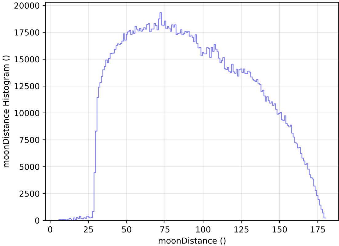
scp_reweight_v3.3_10yrs All sky all bands: moonDistance Histogram
